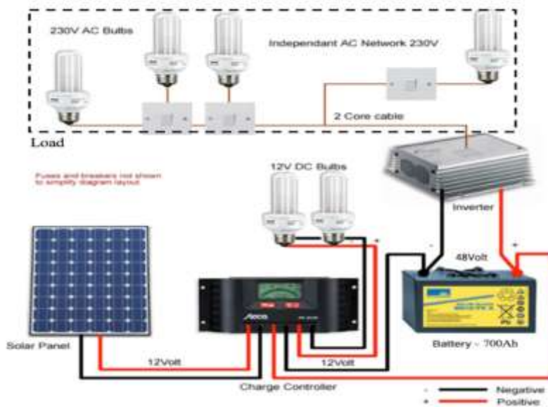
Fig. 2. Stand-alone PV system (off-Grid)
