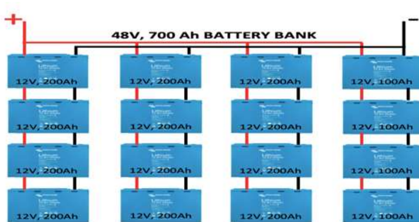
Fig. 2. Schematic Diagram of battery bank connection
