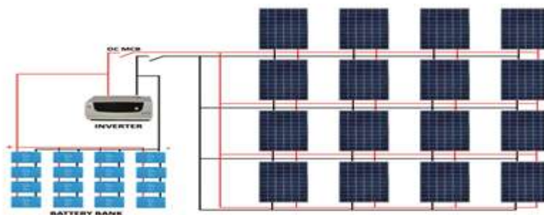
Fig. 1. Schematic Diagram of Panels among with inverters and batteries
