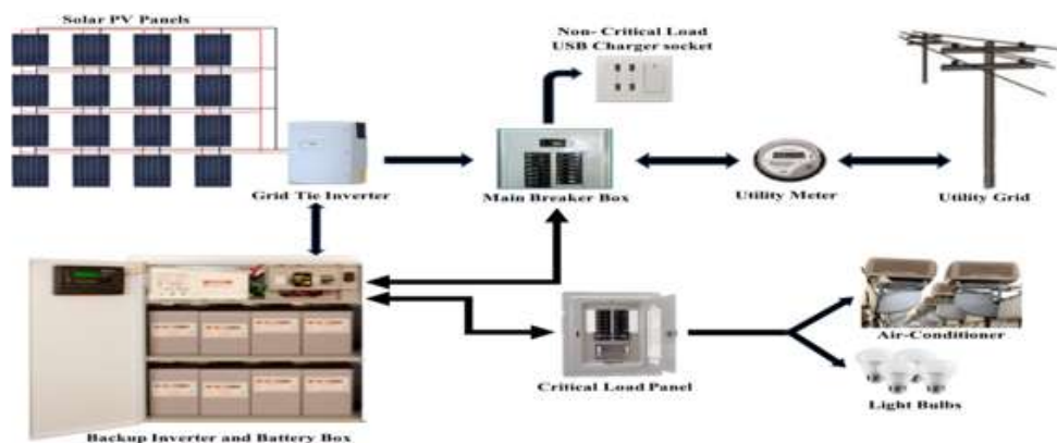
Fig. 3. AC-coupled PV system
