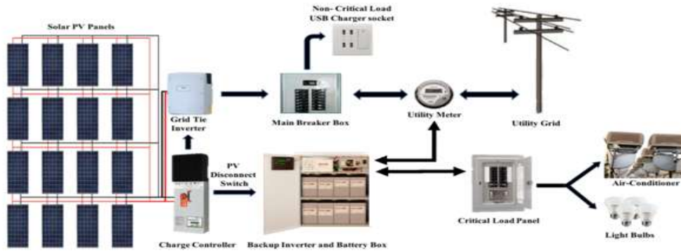
Fig. 5. Dc-coupled PV system
