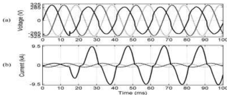
Fig. 10. (a) Voltages at PCC. (b) Fault currents, during the downstream single phase-to-ground arcing fault when the DVR is inactive (bypassed).
