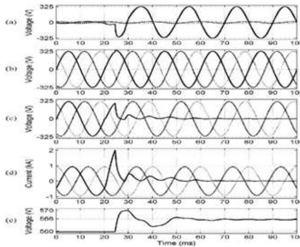
Fig. 9. (a) Injected voltages. (b) Source voltages. (c) Load voltages. (d) Line currents. (e) DC-link voltage, during the single-phase-to-ground down stream fault.
