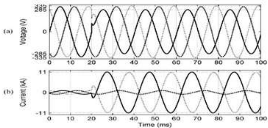
Fig. 6. (a) Voltages at , (b) Fault currents, during downstream phase-to-phase fault when the DVR is inactive (bypassed).
