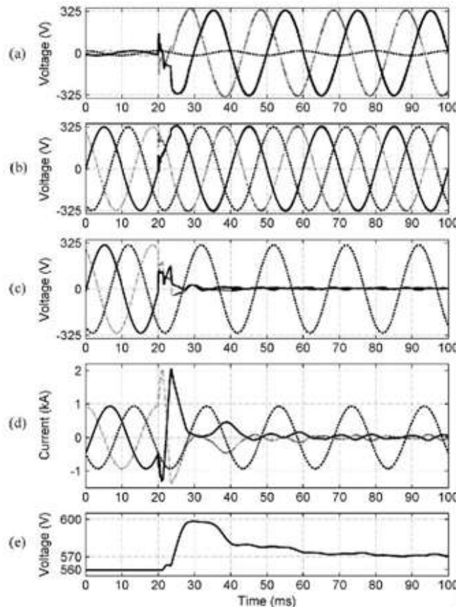
Fig. 7. (a) Injected voltages. (b) Source voltages. (c) Load voltages. (d) Line currents. (e) DC-link voltage, during the phase-to-phase downstream fault.
