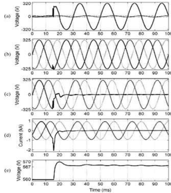
Fig. 11. (a) Injected voltages. (b) Source voltages. (c) Load voltages. (d) Line currents. (e) DC-link voltage, during the single-phase-to-ground down stream arcing fault.
