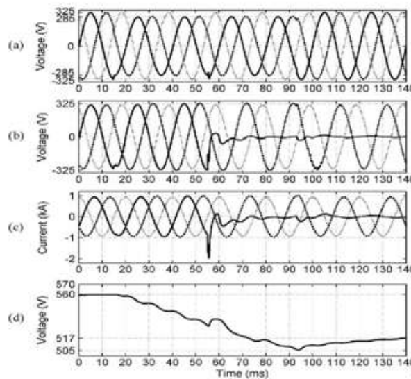
Fig. 12. (a) Source voltages. (b) Load voltages. (c) Line currents. (d) DC-link voltage, during phase-A to ground downstream fault which takes place during sag compensation in phases A and B.
