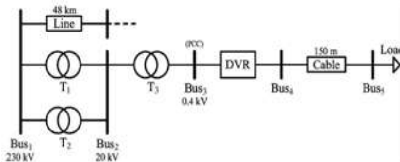
Fig. 3. Single-line diagram of the system used for simulation studies.
