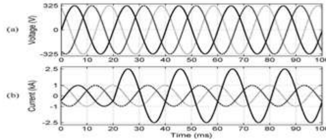
Fig. 8. (a) Voltages at PCC. (b) Fault currents, during the downstream single phase-to-ground fault when the DVR is inactive (bypassed).
