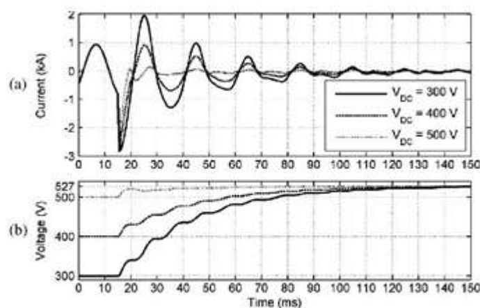
Fig. 13. (a) Line current of phase-A and (b) dc-link voltage, for different initial values of the dc-link voltage, during downstream phase-A-to-ground fault.
