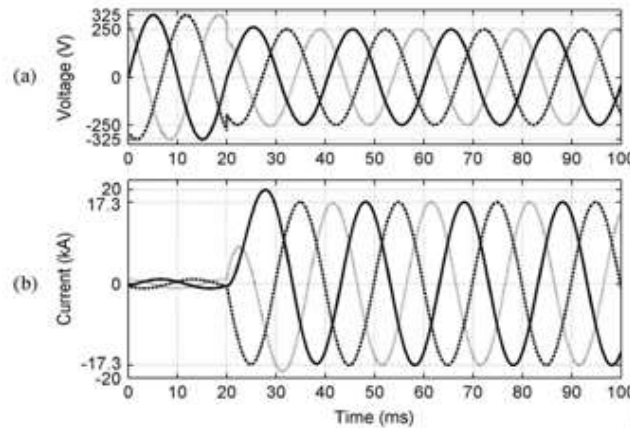
Fig. 4. (a) Voltages at . (b) Fault currents, during downstream three-phase fault when the DVR is inactive (bypassed).
