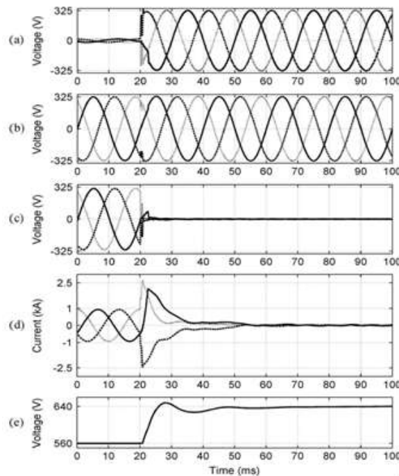
Fig. 5. (a) Injected voltages. (b) Source voltages. (c) Load voltages. (d) Line currents. (e) DC-link voltage, during the three phase downstream fault.
