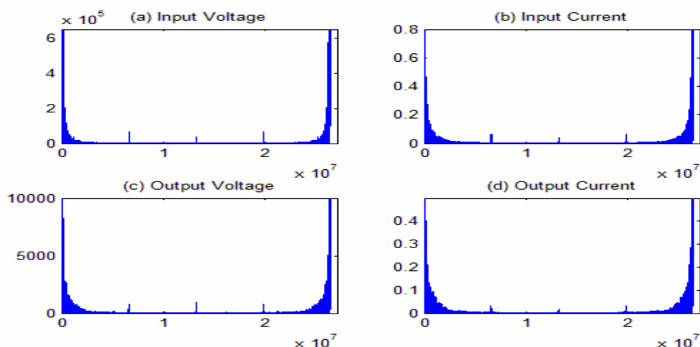
Fig. 2 FFT plot of input and output voltage and current signals in a turn-to-turn short circuit fault between the second and the third turns of the primary winding in with-load mode.
