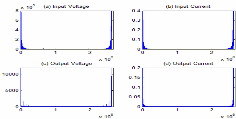
Fig. 3 FFT plot of input and output voltage and current signals in a turn-to-turn short circuit fault between the first and the second turns of the secondary winding in with-load mode.
