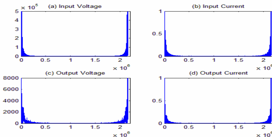
Fig. 1 FFT plot of input and output voltage and current signals in a turn-to-turn short circuit fault between the first and the second turns of the primary winding in with-load mod
