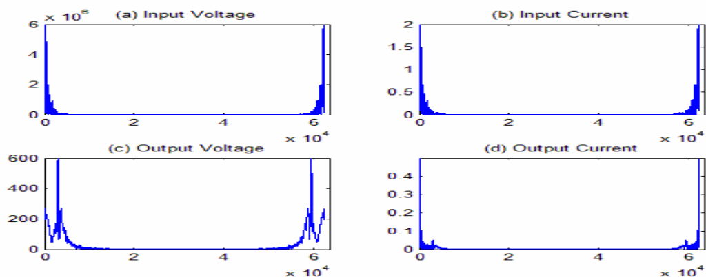
Fig. 5 The first turn of the primary winding is short circuited to the first turn of the secondary winding in with-load mode. Fig.
