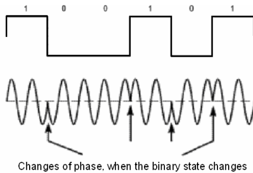
Fig 2: BPSK modulator output
