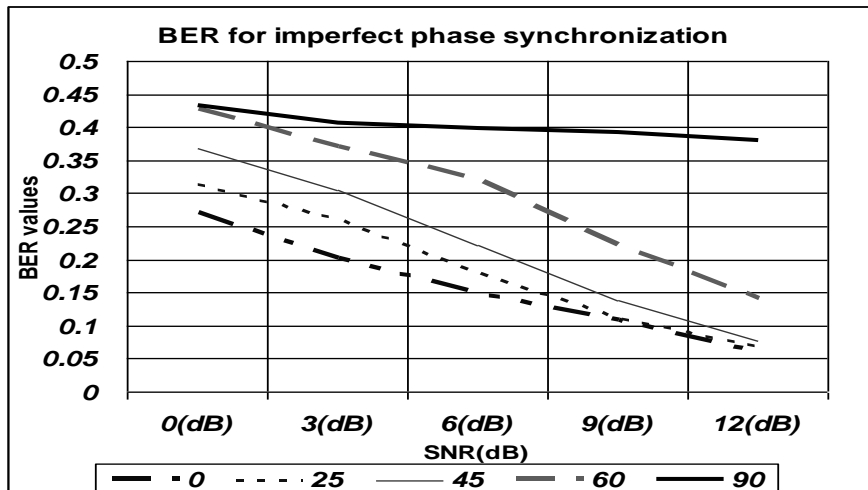
Fig 7: Simulation results of Modulation and Demodulation process.
