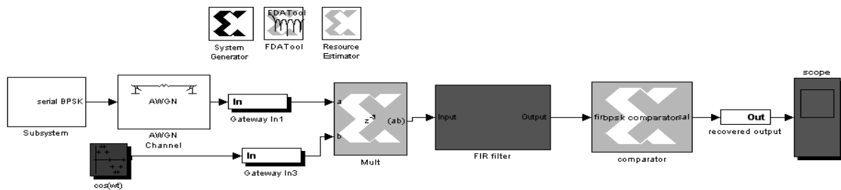
Fig 6: BPSK detector using system generator.
