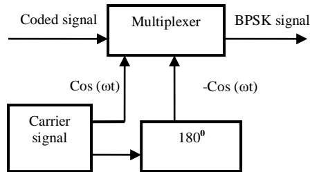
Fig 1: BPSK modulator
