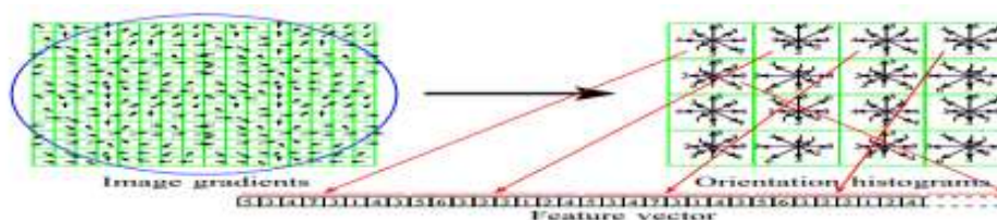
Fig 4. The computation of the feature vector of a key point [12].
