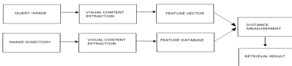
Fig 1: Block diagram of Content Based Image Retrieval.
