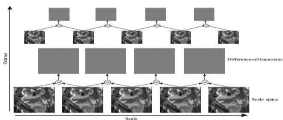
Fig 2: The construction of scale space extrema based on difference-of-Gaussians. [12]
