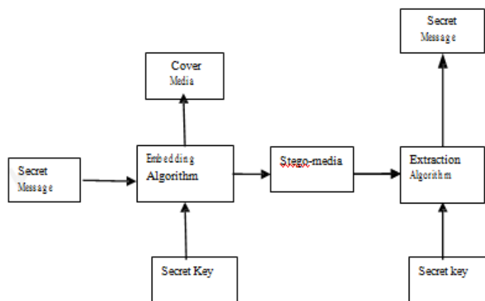
A. Fig 1 Basic steganographic process
