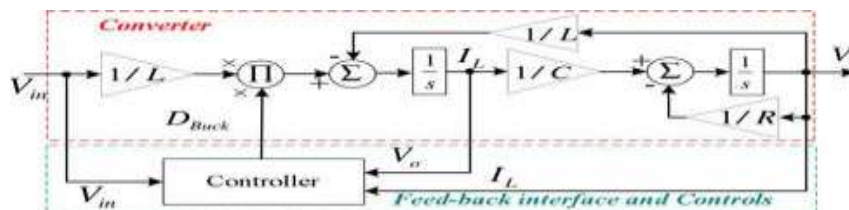
Fig. 8. State-space model of the simplified converter in buck mode Whereas D_1 , D_4 , and D_5 are reverse-biased and do not conduct. In this mode, V_{batt} and V_{dc} are sequentially the input and output voltages. The dc link voltage can be regulated in driving mode (regenerative braking) by controlling the current drawn from the battery. In plug-in charging mode, the current or power drawn from battery is also controllable.
