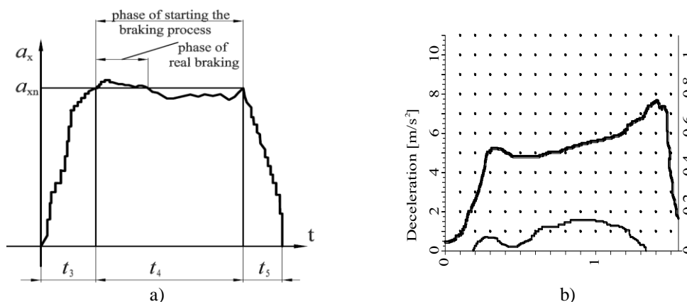
Fig. 4 - Diagram of braking without ABS a) phase of starting the braking process b) phase of real braking
