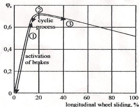
Fig. 1b -The response of the coefficient of cohesion of tyres with the surface of the road
