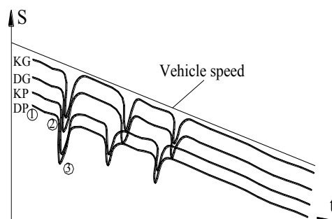
Fig. 1a - Variation of speed in relation to the braking time
