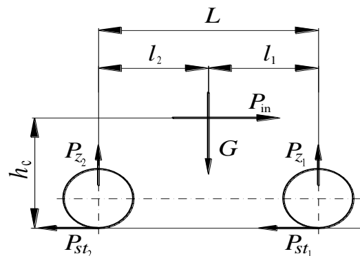
Fig. 2 - Scheme of forces in the process of braking without wheels blocking
