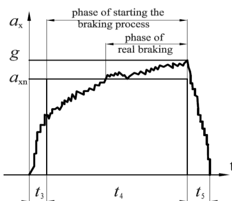
Fig. 3 - Diagram of braking with ABS-phase of starting the braking process
